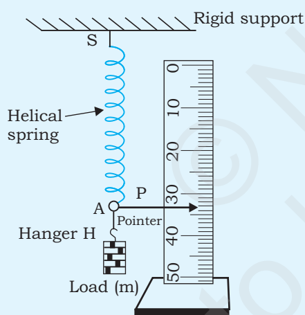
Fig. P 9.1: Measurement of extension of a helical spring due to a load
